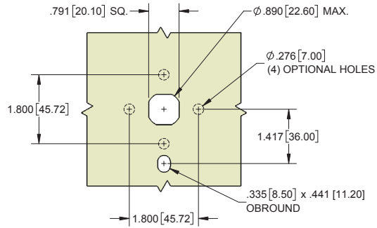
MOUNTING DIMENSIONS
