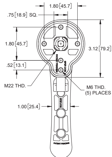
MOUNTING DIMENSIONS
