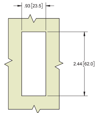
MOUNTING DIMENSIONS FOR .04 [1.0] - .16 [4.0] PANEL THICKNESS
