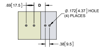
MOUNTING DIMENSIONS
