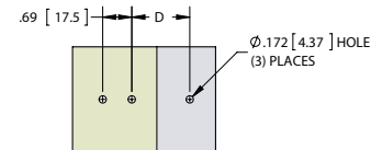
MOUNTING DIMENSIONS
