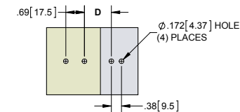
MOUNTING DIMENSIONS
