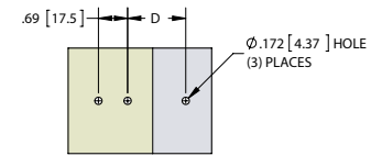
MOUNTING DIMENSIONS
