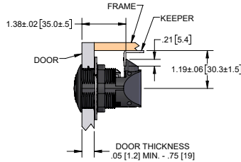
SIDE VIEW CUT-OUT DETAILS
