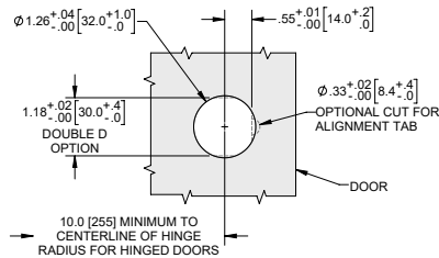
FRONT VIEW DOOR CUT-OUT DETAILS
