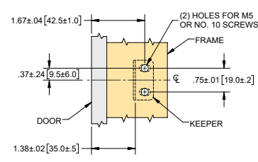
TOP VIEW KEEPER MOUNTING DETAILS
