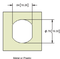
MOUNTING DIMENSIONS
