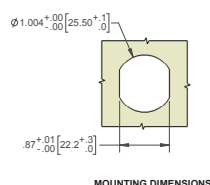
MOUNTING DIMENSIONS
