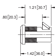
LATCH
