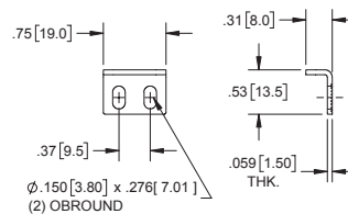
STRIKE
