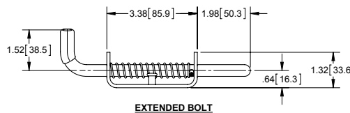
EXTENDED BOLT
