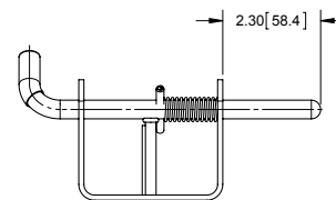
EXTENDED BOLT
