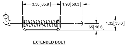
EXTENDED BOLT
