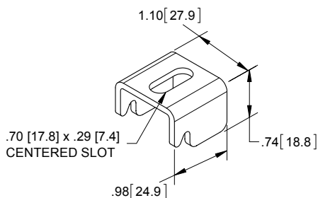
Clamp Bracket Details
