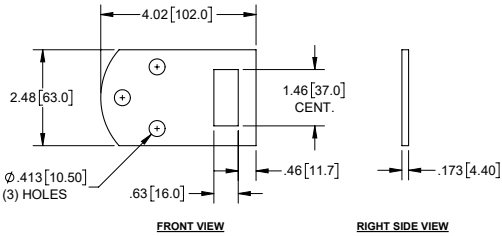
CORNER KEEPER
