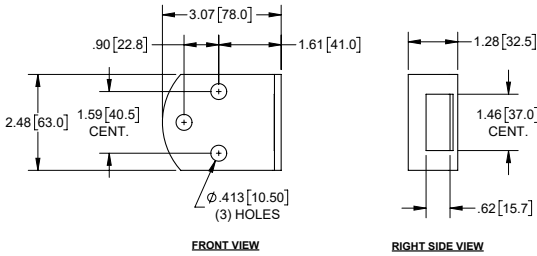
FLUSH KEEPER
