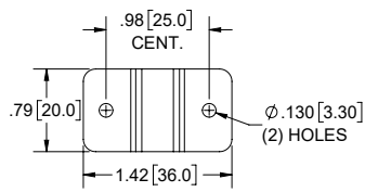
STRIKER BOTTOM VIEW
