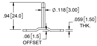
STRIKER TOP VIEW
