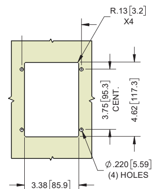
MOUNTING DIMENSIONS
